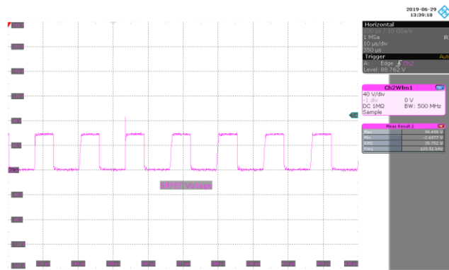
Figure 77 – 120 VAC 60 Hz, Full Load Normal. V_{SRFET} , 40 V / div., 10 \mu s / div.
