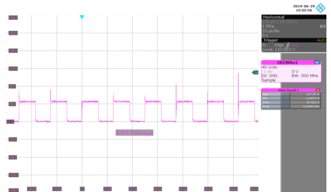
Figure 73 – 90 VAC 60 Hz, Full Load Normal. V_{SRFET} , 40 V / div., 10 \mu s / div.
