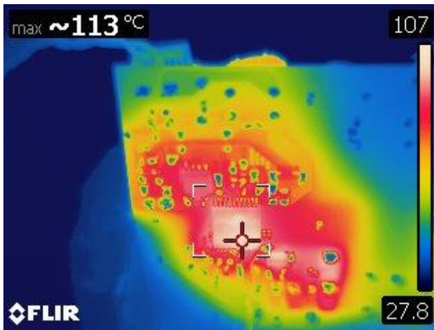
Figure 19 – LYTSwitch-6 (U4).
