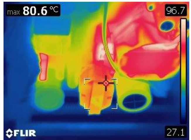
Figure 22 – PFC Inductor (T1).
