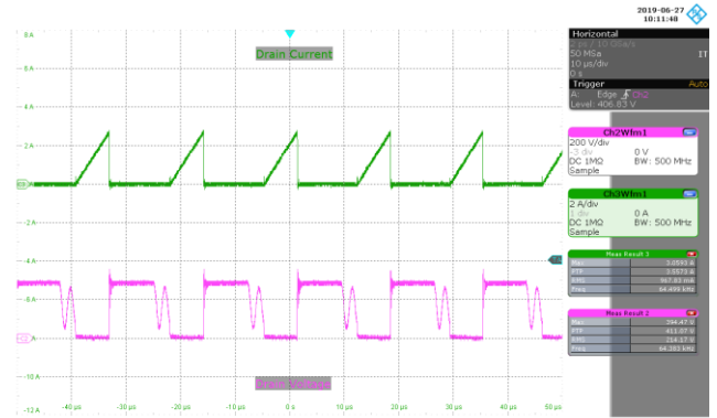
Figure 45 – 120 VAC 60 Hz, Full Load Normal. Upper: I_{DRAIN} , 2 A / div. Lower: V_{DRAIN} , 200 V / div., 10 \mu s / div.
