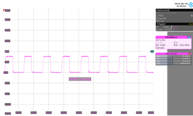
Figure 79 – 132 VAC 60 Hz, Full Load Normal. V_{SRFET} , 40 V / div., 10 \mu s / div.
