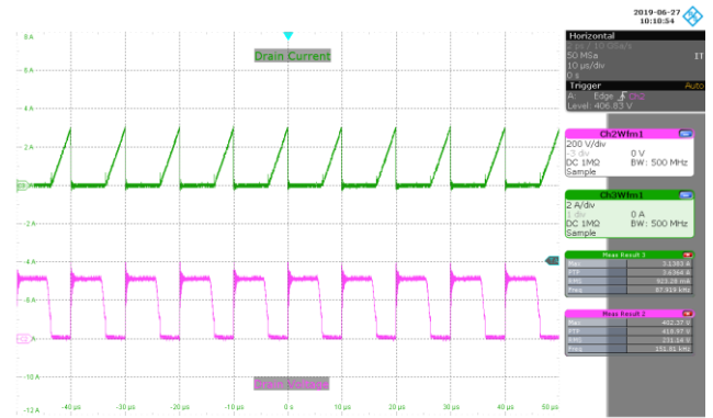
Figure 47 – 132 VAC 60 Hz, Full Load Normal. Upper: I_{DRAIN} , 2 A / div. Lower: V_{DRAIN} , 200 V / div., 10 \mu s / div.
