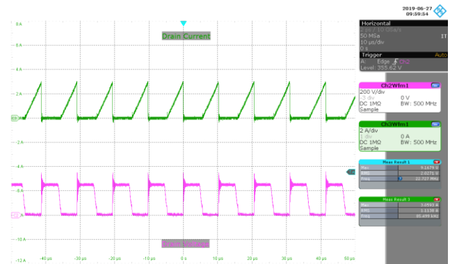
Figure 41 – 90 VAC 60 Hz, Full Load Normal. Upper: I_{DRAIN} , 2 A / div. Lower: V_{DRAIN} , 200 V / div., 10 μs / div.
