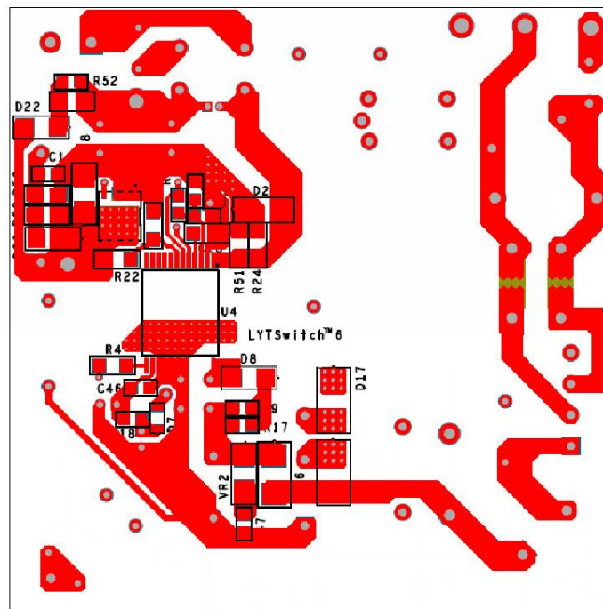
Figure 6 – Main Board Bottom Side.
