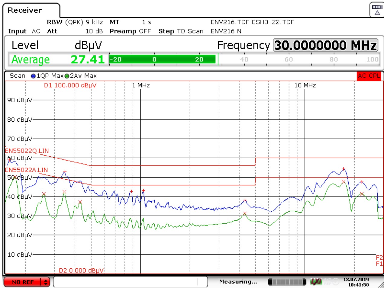
Figure 87 – Conducted EMI QP Scan at Full Load, Earthed, 120 VAC 60 Hz and EN55022 B Limits.
