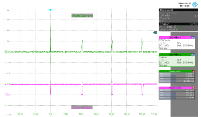
Figure 55 – 132 VAC 60 Hz, Full Load Start-up. Upper: I_{DRAIN} , 2 A / div. Lower: V_{DRAIN} , 200 V / div., 20 μs / div.
