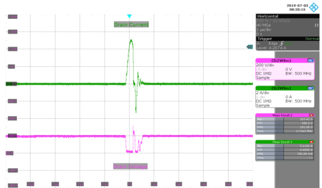
Figure 61 – 120 VAC 60 Hz, Output Shorted. Upper: I_{DRAIN} , 2 A / div. Lower: V_{DRAIN} , 200 V / div., 1 \mu s / div.
