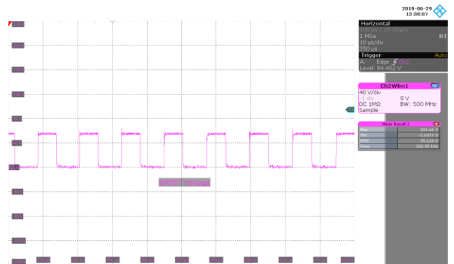
Figure 75 – 110 VAC 60 Hz, Full Load Normal. V_{SRFET} , 40 V / div., 10 \mu s / div.
