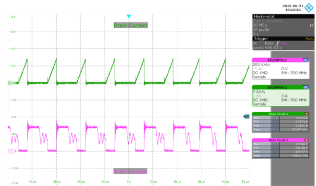
Figure 43 – 110 VAC 60 Hz, Full Load Normal. Upper: I_{DRAIN} , 2 A / div. Lower: V_{DRAIN} , 200 V / div., 10 μs / div.
