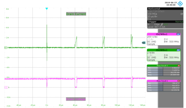
Figure 53 – 120 VAC 60 Hz, Full Load Start-up. Upper: I_{DRAIN} , 2 A / div. Lower: V_{DRAIN} , 200 V / div., 20 μs / div.
